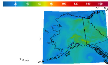
8Hr Avg Ozone Concentration(PPB) Ending Tue Jul 05 2011 7PM EDT (Tue Jul 05 2011 23Z) National Digital Guidance Database 12z model run Graphic created-Jul 05 12:29PM EDT
