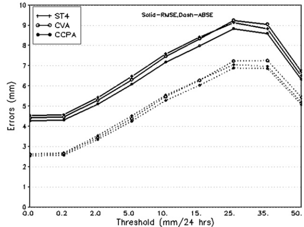
FIG. 14. RMSE (solid line) and ABSE (dotted line) of 24-h precipitation from Stage IV (cross), CVA (open circle), and CCPA (closed circle) verified against RFC rain gauge analysis at the 0.125^\circ grid, as a function of precipitation threshold.
