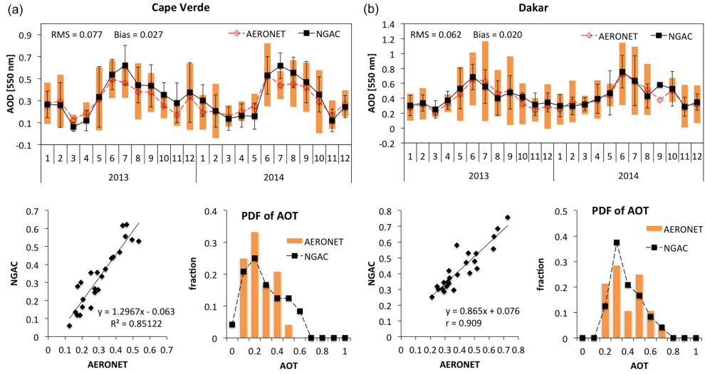
Figure 6. (a) NGAC V1.0 vs. L1.5 AERONET 550-nm AOD comparisons at Cape Verde for the 2013–2014 period: a time series, scatterplot, and fractional distribution histogram. In the time series, the model monthly means and standard deviation about the mean are shown in the black symbols and lines. The AERONET monthly means and standard deviation about the mean are shown in the red shading and orange bars. In the PDF plot, the model is indicated by the black symbols and line, and the AERONET observations are indicated by orange bars. We thank Didier Tanre for the efforts in establishing and maintaining Cape Verde and Dakar sites. (b) NGAC V1.0 vs. AERONET 550 nm AOD comparisons at Dakar for the 2013–2014 period: a time series, scatterplot, and fractional distribution histogram.
