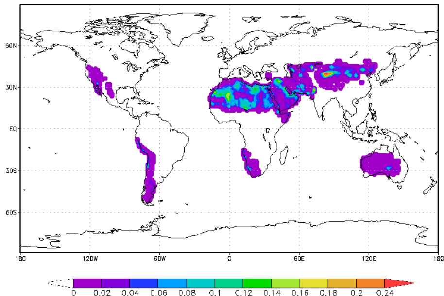
GOCART Dust Source Function
