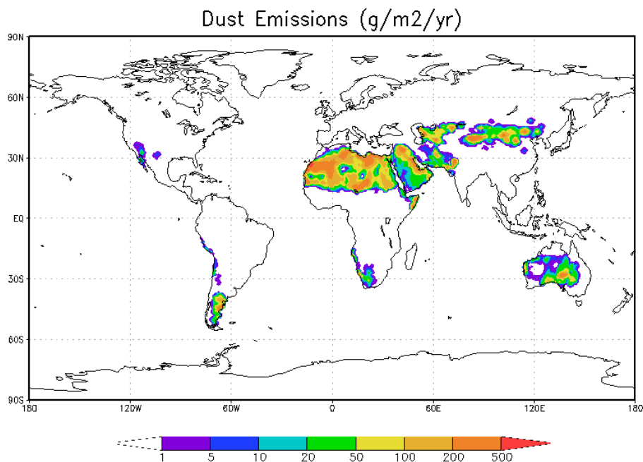
Figure 4. Annual dust emissions (in \text{g}/\text{m}^2/\text{yr}^{-1} ) over the September 2012–September 2013 period.
