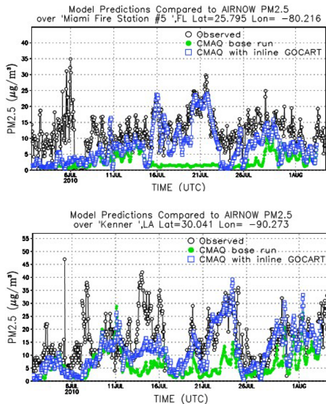
Figure 9. Time series of PM 2.5 from EPA AIRNOW observations (black dot), CMAQ baseline run using static LBCs (green dot) and CMAQ experimental run using NGAC LBCs (blue square) at Miami, FL (top panel) and Kenner, LA (bottom panel).
