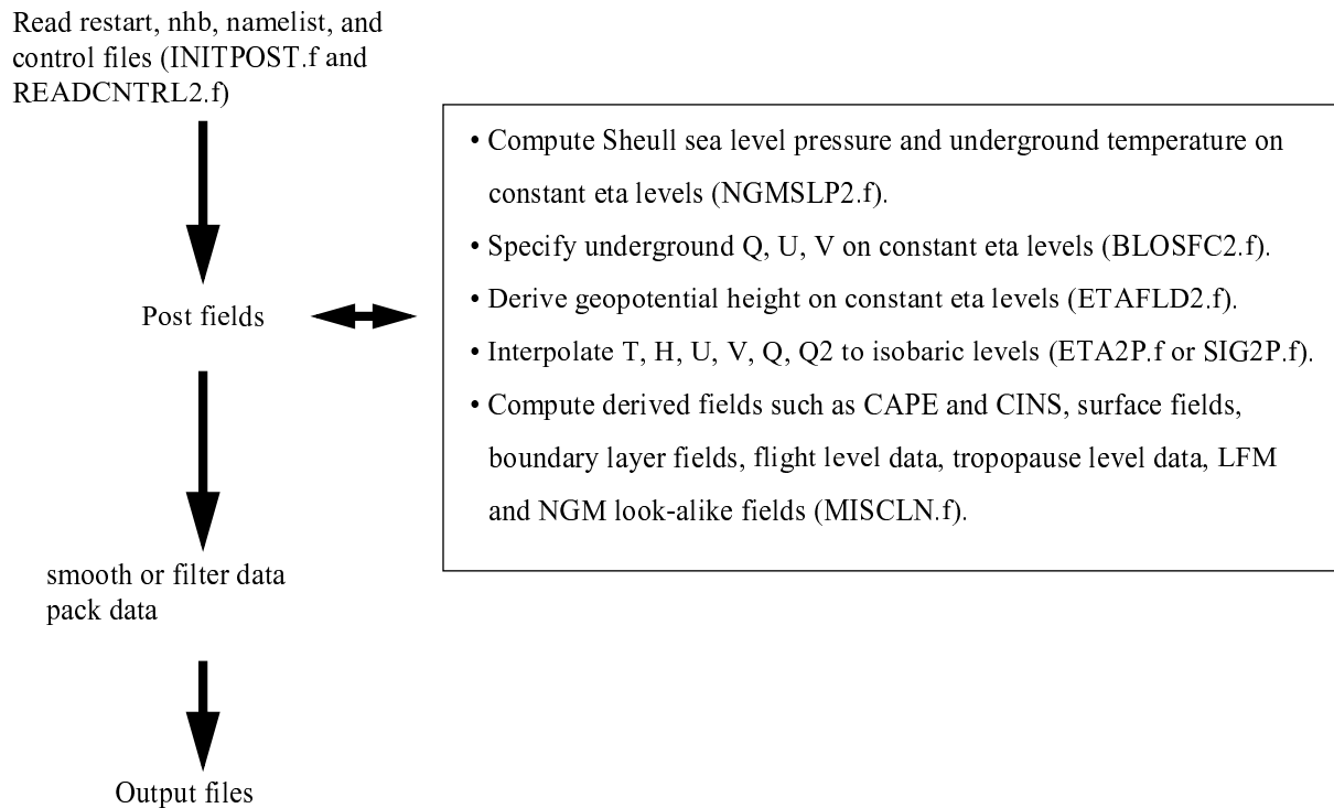
Fig. 3. Schematic of flow through post processor.
