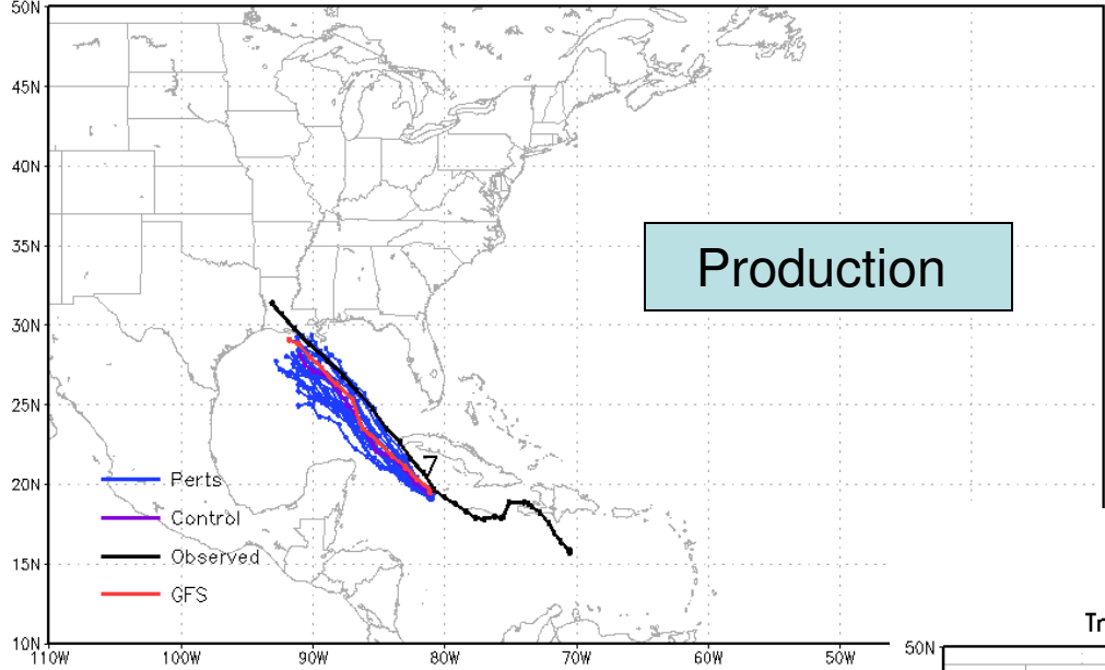
Tropical Cyclone Forecast Tracks – prod NCEP Ensemble – 2008083000
