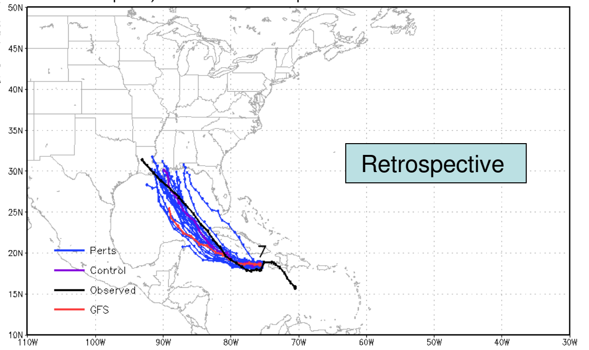
Tropical Cyclone Forecast Tracks – para NCEP Ensemble – 2008082800
