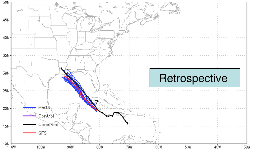
Tropical Cyclone Forecast Tracks – para NCEP Ensemble – 2008083000
