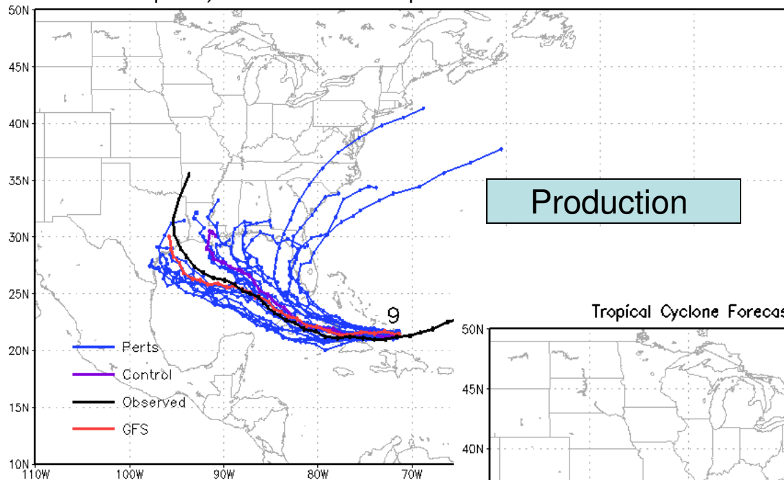
Tropical Cyclone Forecast Tracks – prod NCEP Ensemble – 2008090700
