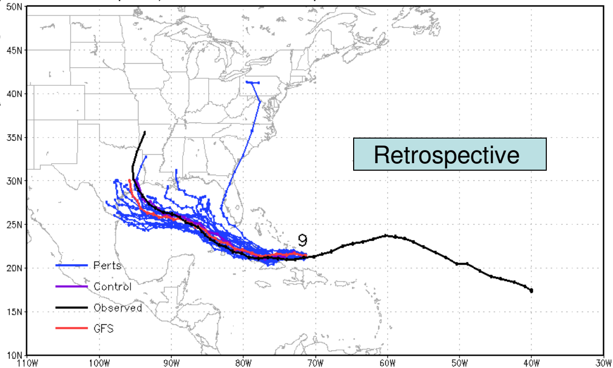
Tropical Cyclone Forecast Tracks – para NCEP Ensemble – 2008090700
