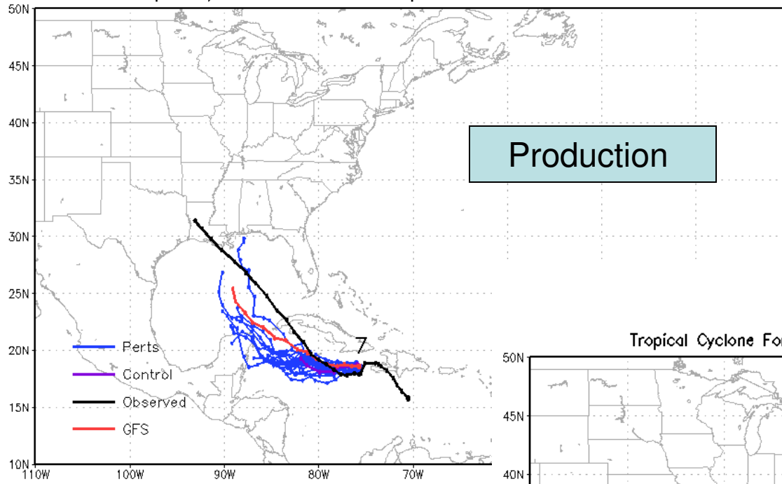
Tropical Cyclone Forecast Tracks – prod NCEP Ensemble – 2008082800
