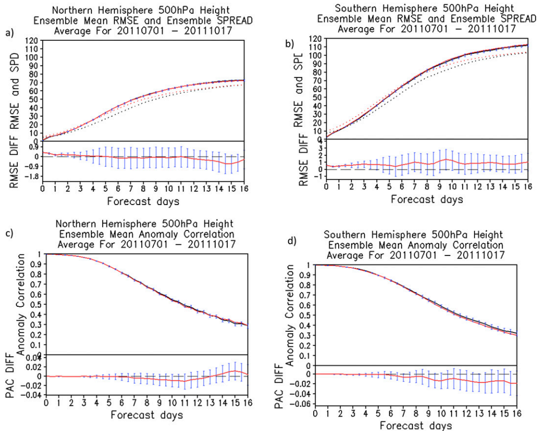
FIG. 5. Ensemble mean RMSE (solid) and ensemble standard deviation (dotted) for 500-hPa geopotential height over the (a) NH and (b) SH. The verification scores for ETR_ONLY (black) and EnKF_ONLY (red) are averaged during the period from 1 Jul to 17 Oct 2011. The bottom portion of each panel shows the difference in RMSE error (EnKF minus ETR). The blue bars display the 95% confidence intervals with the bootstrap significant test. (c),(d) As in (a),(b), but for the 500-hPa geopotential height ensemble mean predicted pattern anomaly correlations.
