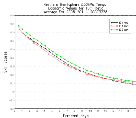
Fig. 10. REV (10:1 cost/loss ratio) for the NCEP 14 global ensemble raw forecast (black) compared to the CMC 16 global raw forecast (red) and the combined NCEP and CMC ensemble (green) for NH extra-tropical 850hPa temperature for the winter of 2006-2007.
